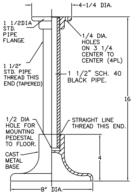
PEDESTAL REQUIREMENTS PER BENCH. 4 REQ'D.
